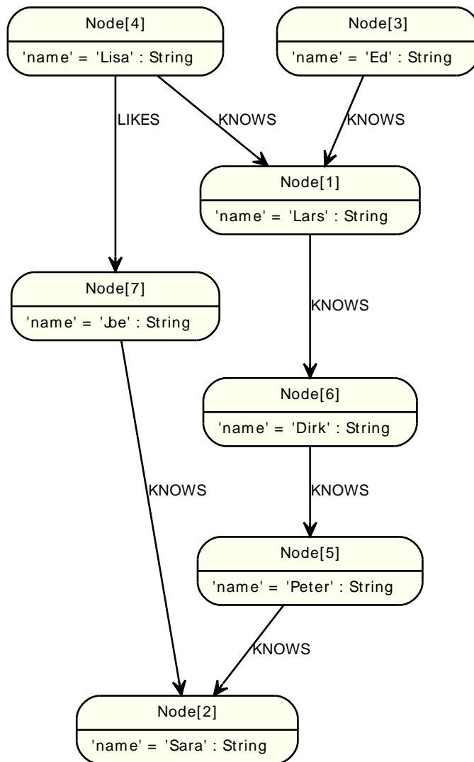
Figure 8.1. Traversal Example Graph
