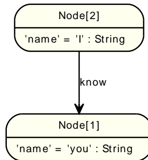
Figure 29.1. Hello World Graph
