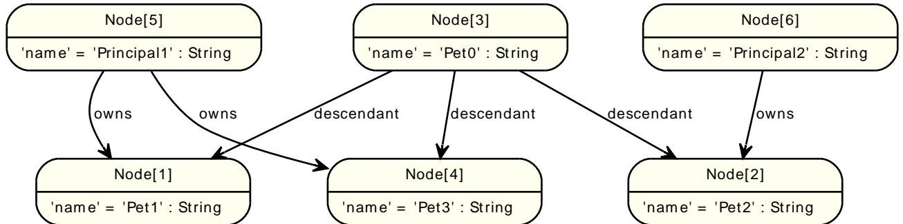
Figure 4.4. Descendants Example Graph
