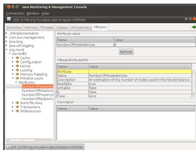
Figure 25.2. Neo4j MBeans View
